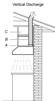
A. 7" (17.8 cm) round vent. B. Cabinet C. Roof cap with damper (not included).
