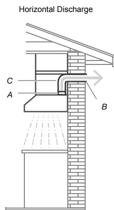
A. 7" (17.8 cm) round vent. B. Wall cap with damper (not included). C. 90° elbow
